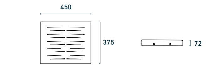
Vista Frontal
