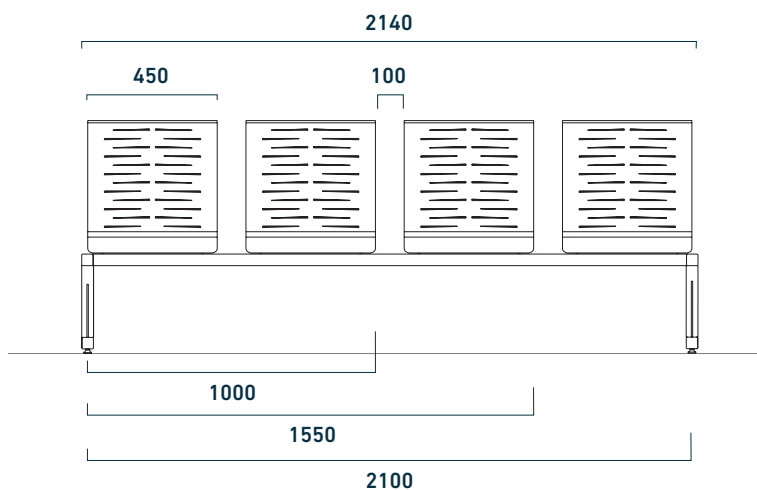
Vista Frontal
